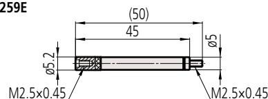
Extension rod 21AAA259E
